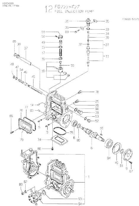
OCD10-M43900 ENGINE 3TNC78L-RTBA Fig.12. FUEL INJECTION PUMP
