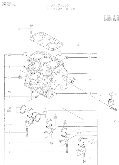
Fig.1. CYLINDER BLOCK
